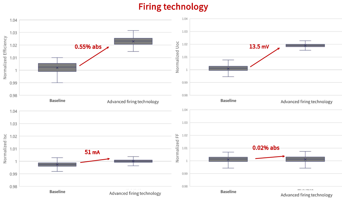
Figure 3. Industry-leading firing technology improves TOPCon cell performance
