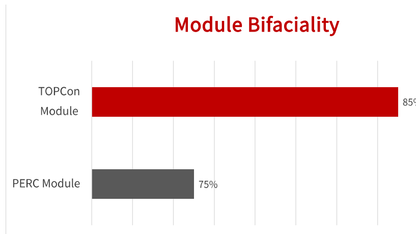
Figure 5. Bifaciality of PERC and TOPCon modules
