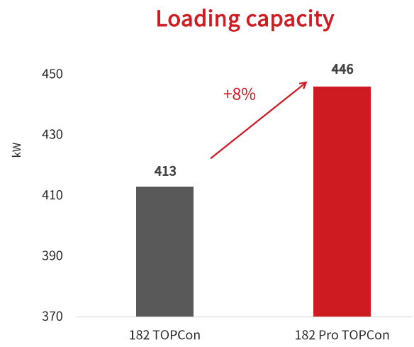
Figure 9. Loading capacity comparison between 182 TOPCon and 182 Pro TOPCon
